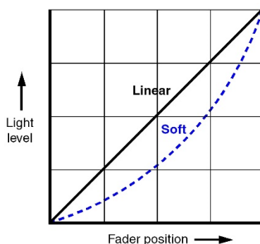
Figure 2. Dimming curves
