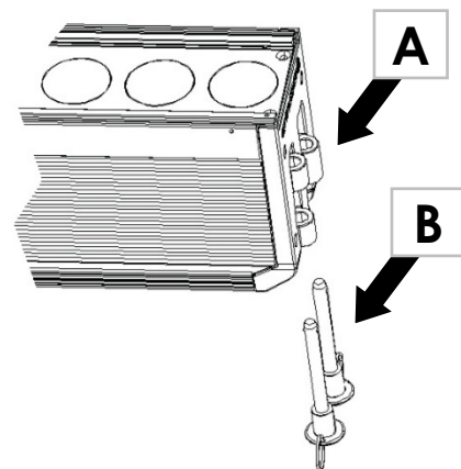
Figure 9. End channels and locking pins
