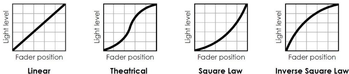
Figure 16. Dimming curves
