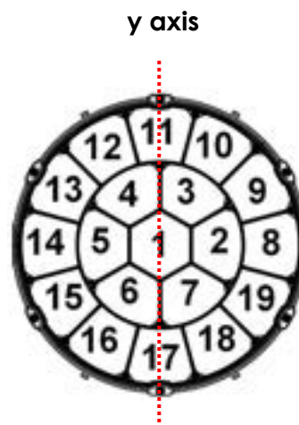
y-mirror pixel layout
